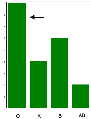
Bar Chart / Bar Graph for Blood Type
